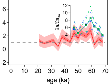
VM29-19 Rashid et al. [2011]
