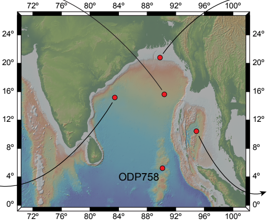
MD77-169 Colin et al. [1999]
