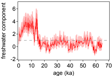
MD77-169 Colin et al. [1999]
