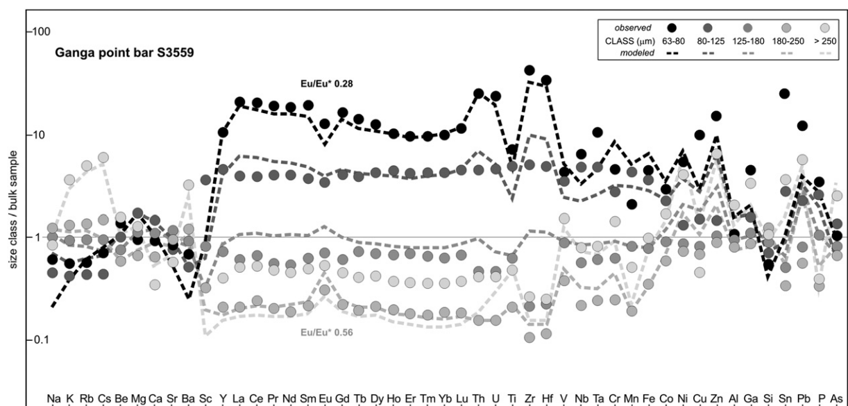
Fig. 7. Modeled versus observed intrasample chemical variability in Ganga bar sample S3559 (elements in multi-element diagram normalized to bulk-sample composition). The model reproduces observed trends for most elements. Alkali and alkaline-earth metals, hosted in tectosilicates and phyllosilicates, are enriched in the coarse tail; Y, REE, Th, U, Zr, and Hf, hosted in ultradense zircon, monazite, allanite, and garnet are enriched in the fine tail (but increase again in the mica-dominated coarsest tail). Note hydraulic control on the Eu anomaly, most strongly negative in the finest tail.
