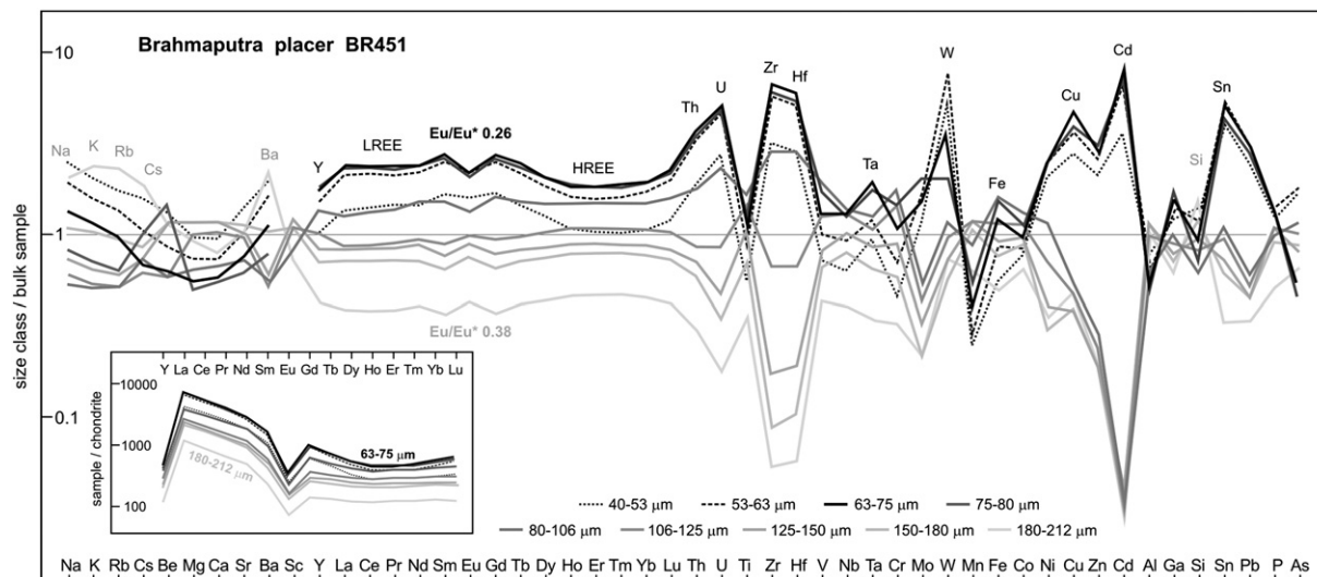
Fig. 5. Intrasample chemical variability in Brahmaputra placer BR451 (elements in multi-element diagram normalized to bulk-sample composition and arranged following the periodic table group by group). Inset shows chondrite-normalized YREE patterns. Because of the settling-equivalence effect, Na, K, Rb, Cs, Ba, and Si are concentrated in the tectosilicate-rich upper-fine-sand class, and Y, REE, Th, U, Ti, Zr, Hf, V, Nb, Ta, Cr, W, Fe, Ni, Cu, Zn, Cd, and Sn in heavy-mineral-rich very-fine sand classes (but less so in very-coarse silt classes largely including finer modes poorer in heavy minerals). Note hydraulic control on the Eu anomaly, most strongly negative in the finest sand class.
