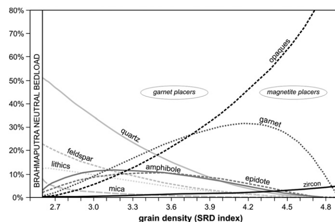
Fig. 8. Predicted mineralogical trends for Brahmaputra bedload. At increasing SRD indices, dense and next ultradense detrital components progressively increase at the expense of mica, quartz, feldspar and lithic grains, to form garnet-rich and finally magnetite-rich placers. Mica decreases at fastest rate to account for easier entrainment of platy grains, as documented by marked phyllosilicate depletion in placer deposits ( Garzanti et al., 2009 ).
