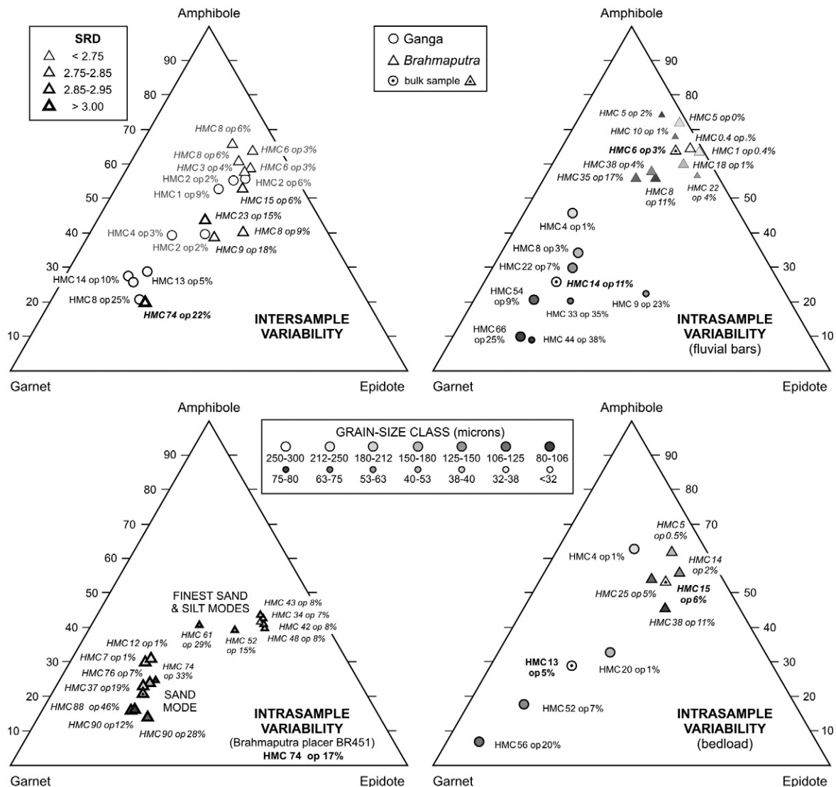
Fig. 2. Intersample and intrasample mineralogical variability. The three dominant mineral groups in collision-orogen detritus have different densities (amphibole \sim 3.2 \text{ g/cm}^3 ; epidote \sim 3.45 \text{ g/cm}^3 ; garnet \sim 4.0 \text{ g/cm}^3 ). Their relative abundance, in different samples and different size classes of each sample, is consequently controlled by hydraulic effects, which dim provenance-related differences (e.g., higher garnet in Ganga sediments). Denser minerals (HMC = Heavy Mineral Concentration; op% = percentage of ultradense opaques on bulk sample) are enriched to different degrees in different samples because of selective-entrainment effects (upper left triangle), and systematically in finer classes of each sample because of settling-equivalence effects (upper right and lower right triangles). The settling-equivalence principle applies to both main sand mode and finer modes (lower left triangle).
