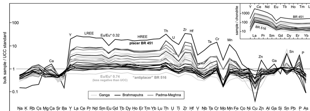
Fig. 3. Intersample chemical variability (elements in UCC-normalized multielement diagram arranged following the periodic table group by group). Inset shows chondrite-normalized YREE patterns. The nearly two-orders-of-magnitude variability in Y, REE, Th, U, Ti, Zr, Hf, Ta, Cr, and Mn (to a lesser extent in Ca, Zn, Ga, Sn, P), with extreme concentration in Brahmaputra placer BR451 and depletion in Ganga "antiplacer" BR516, is a selective-entrainment effect. Depletion in alkali and alkaline-earth metals (Na, Sr, Ba) and Mo is largely a weathering effect. Depletion in Co, Ni, Cu, Zn, Al, Ga, and As in most samples is a suspension-sorting effect (Garzanti et al., in press). Note strict hydraulic control on the Eu anomaly, most strongly negative in placer lags.
