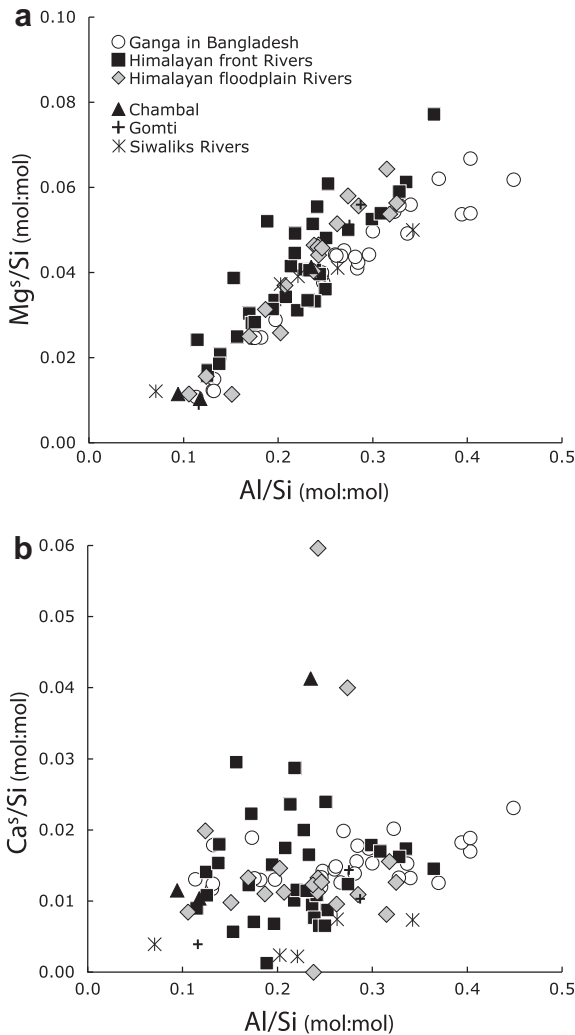
Fig. 11. \text{Mg}^{2+}/\text{Si} (a) and \text{Ca}^{2+}/\text{Si} ratio (b) as a function of \text{Al}/\text{Si} ratio for river sediments from the Himalayan front Rivers, the Himalayan flood plain Rivers, the Ganga in Bangladesh, the Chambal and Gomti Rivers. \text{Mg}^{2+} and \text{Ca}^{2+} are derived from the sediment bulk Mg and Ca content after correction for calcite and dolomite Ca and Mg contribution.
