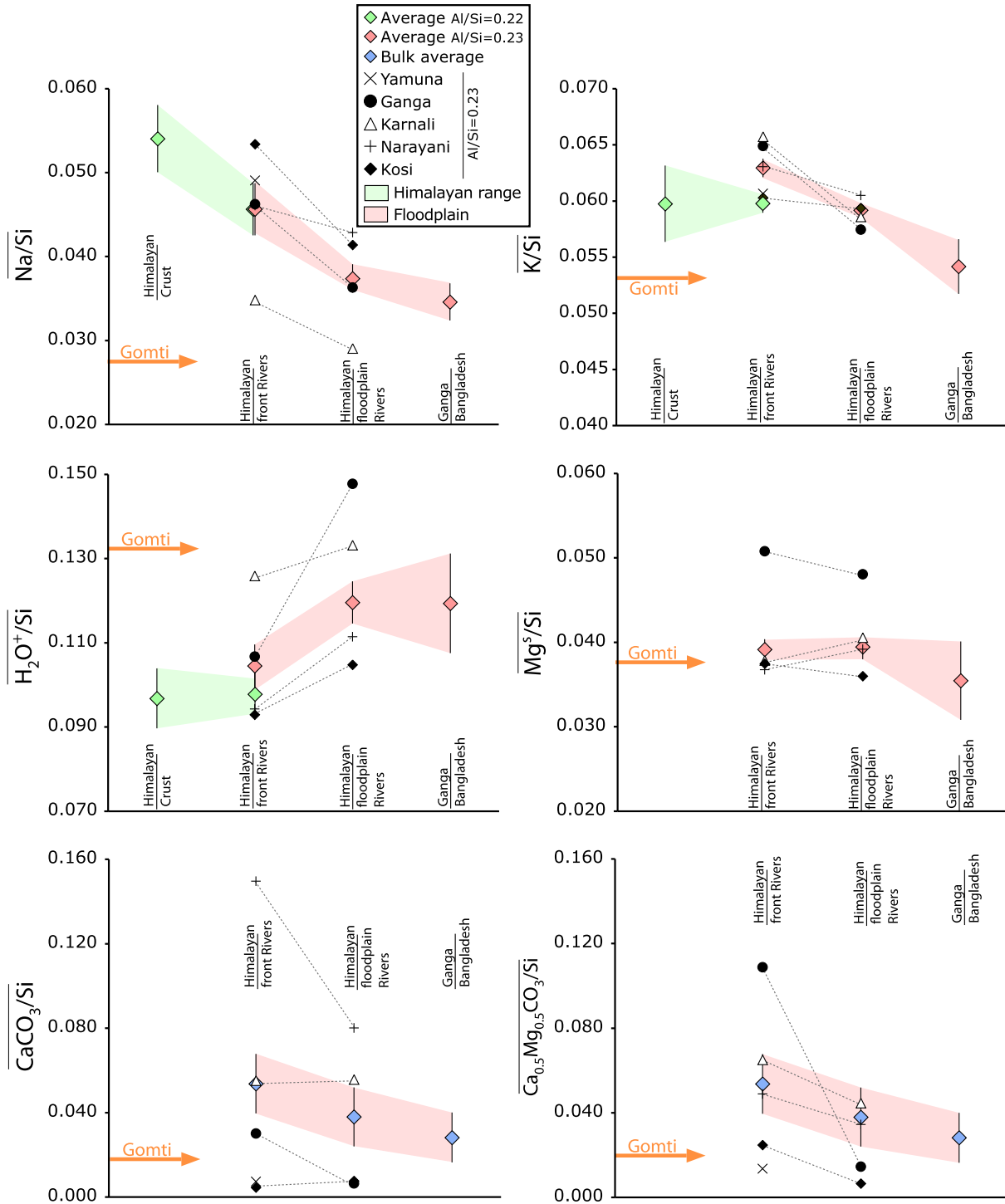
Fig. 13. Evolution of the normalized mobile element composition of sediments in the Himalayan system. Weathering in the Himalayan range (green envelope) is computed for an average \text{Al}/\text{Si} ratio of 0.22. Weathering in the floodplain (red envelope) is determined for an average \text{Al}/\text{Si} ratio of sediments of 0.23 as sequestration in the floodplain leads to an increase in the average \text{Al}/\text{Si} ratio. For carbonates the Si normalized ratios were determined by averaging all available data for each considered river as carbonate content does not show any relation to \text{Al}/\text{Si} . Gomti River sediments as potential analog for floodplain material are also shown for comparison. Details on the calculation can be found in Appendix B. (For interpretation of the references to color in this figure legend, the reader is referred to the web version of this article.)
