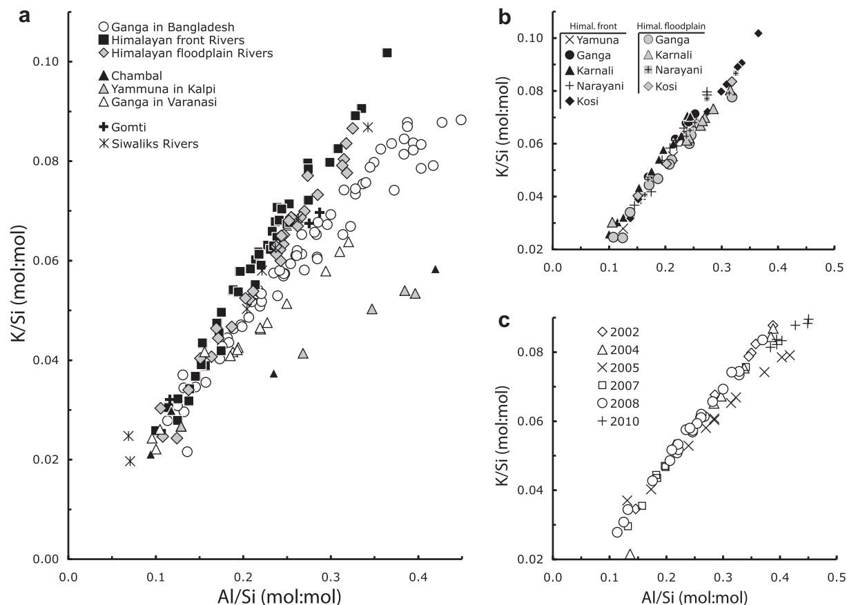
Fig. 6. Evolution of the K/Si ratio as a function of the Al/Si ratio, showing a depletion in K from the Himalayan front Rivers (black squares) downstream to the Himalayan floodplain Rivers (light gray diamonds) and the Ganga in Bangladesh (open circles). (b) Himalayan front River sediments have homogeneous K/Si composition. (c) Inter-annual variability of the K/Si ratio in Ganga sediments sampled in Bangladesh.
