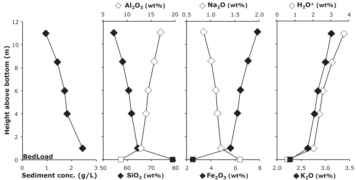
Fig. 2. Evolution of sediment concentration in the water column of the Ganga in Bangladesh (BR 511 – 516) along with the evolution of the chemical composition of major elements Si, Al, Fe, Na, K as well as \text{H}_2\text{O}^+ . Mineral sorting within the water column is a first order control on the chemical composition of sampled sediments (Lupker et al., 2011; Bouchez et al., 2011a).
