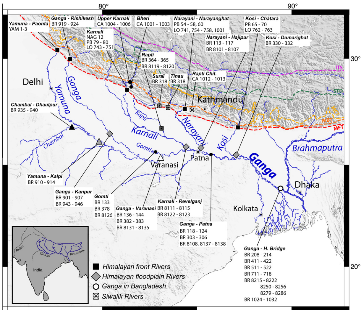
Fig. 1. Geographical setting of the Ganga basin showing the main sample sites and corresponding sample numbers. A geological sketch of the main Himalayan faults zones is also shown (ITS: Indus-Tsangpo Suture; STD: South Tibetan Detachment; MCT: Main Central Thrust; MBT: Main Boundary Thrust; MFT: Main Frontal Thrust).
