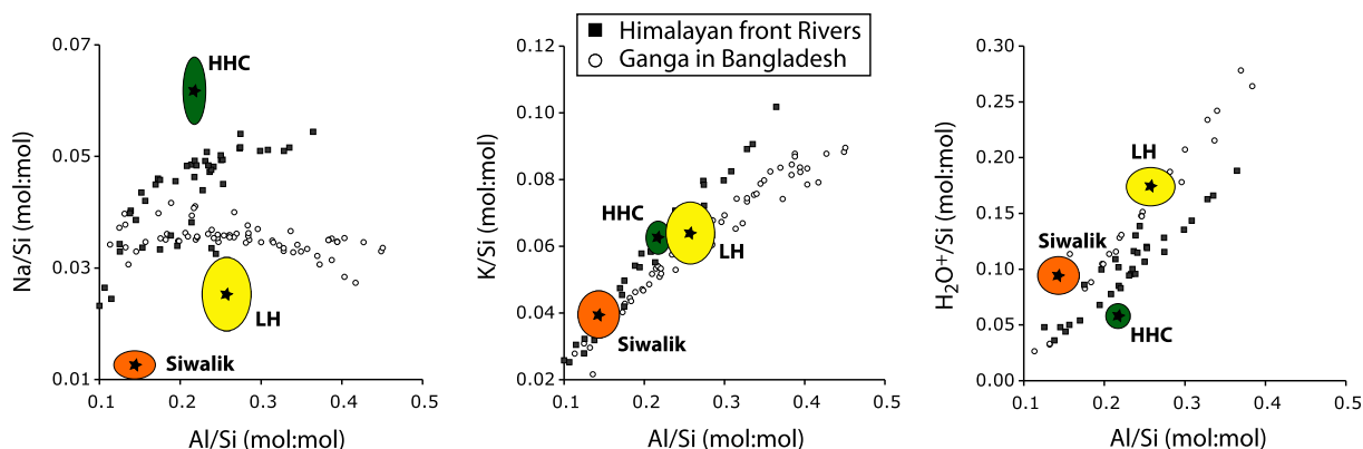
Fig. 12. Na/Si, K/Si and \text{H}_2\text{O}^+/\text{Si} ratios of the main lithological units of the Himalayan orogen: Siwaliks, Lesser Himalaya (LH) and High Himalaya Crystallines (HHC). The chemical composition of these units are from Galy and France-Lanord (2001) and Lupker et al. (2011) and are based on outcrop samples.
