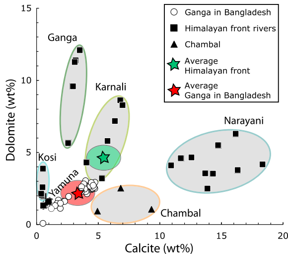
Fig. 9. Calcite and dolomite content of sediments from the Ganga basin.
