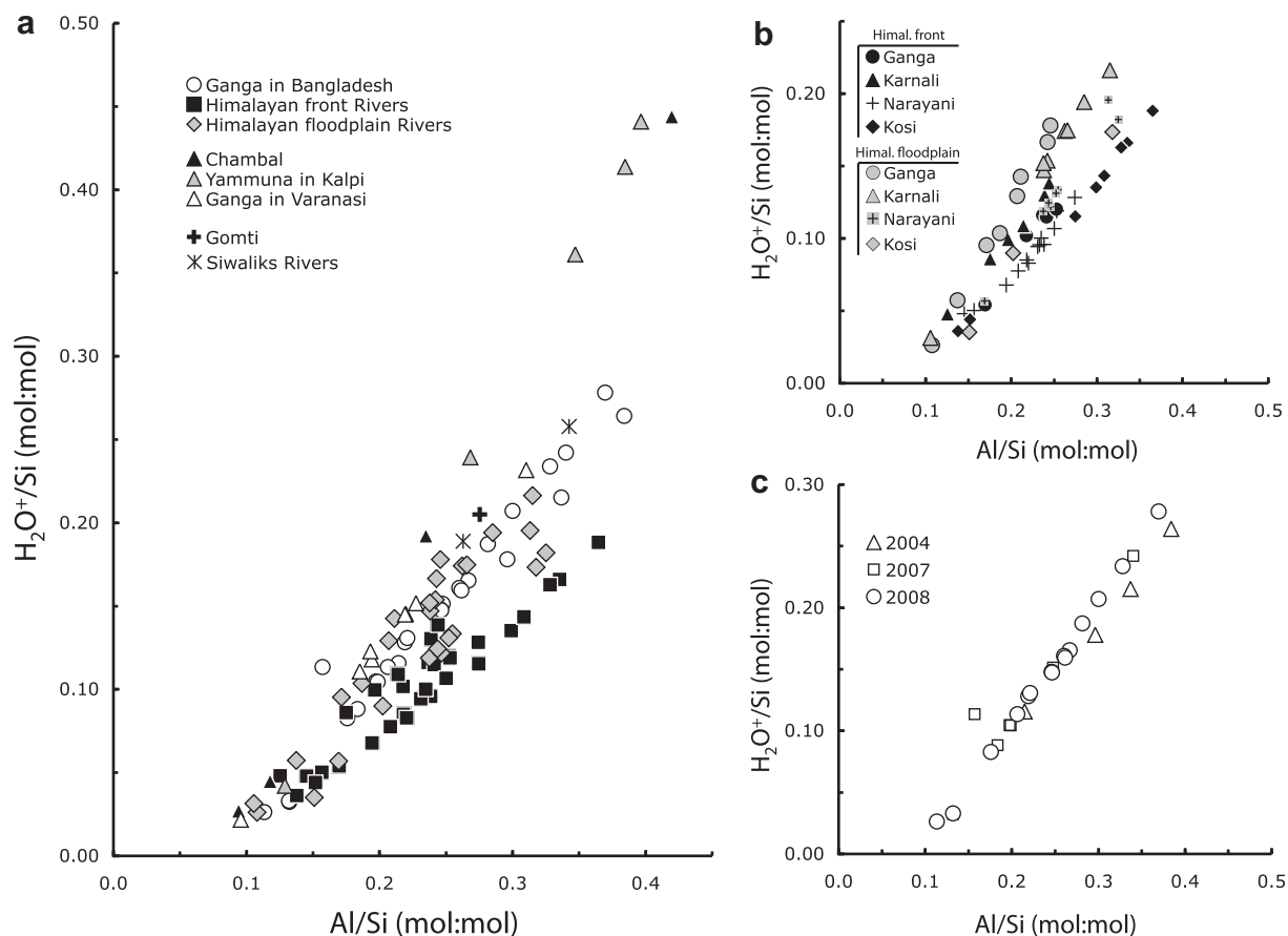
Fig. 7. Evolution of the \text{H}_2\text{O}^+/\text{Si} ratio as a function of the \text{Al}/\text{Si} ratio. (a) Evolution of \text{H}_2\text{O}^+/\text{Si} from the Himalayan front rivers (black squares), further downstream upon floodplain transfer (light gray diamonds) compared to Ganga sediments sampled in Bangladesh (open circles) and the major southern contribution of the Chambal (black triangles). (b) Detailed plot of the evolution of Himalayan rivers upon floodplain transfer. (c) Inter-annual variability of the \text{H}_2\text{O}^+/\text{Si} ratio in Ganga sediments sampled in Bangladesh.
