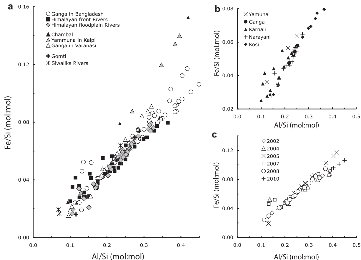
Fig. 4. (a) Evolution of the Fe/Si ratio as a function of the Al/Si ratio, proxy for grain-size and mineral sorting in the river water column. Himalayan Rivers form a relatively uniform trend that is markedly different from sediments from the southern tributaries such as the Chambal. This difference can be used to trace inputs from Chambal sediments in sediments from the Ganga mainstream. (b) Detailed graph of the Himalayan front rivers. (c) Temporal of Fe/Si ratios of sediments sampled in the Ganga in Bangladesh, plotted as a function of sampling year, highlighting the heterogeneity of the exported chemical signal.
