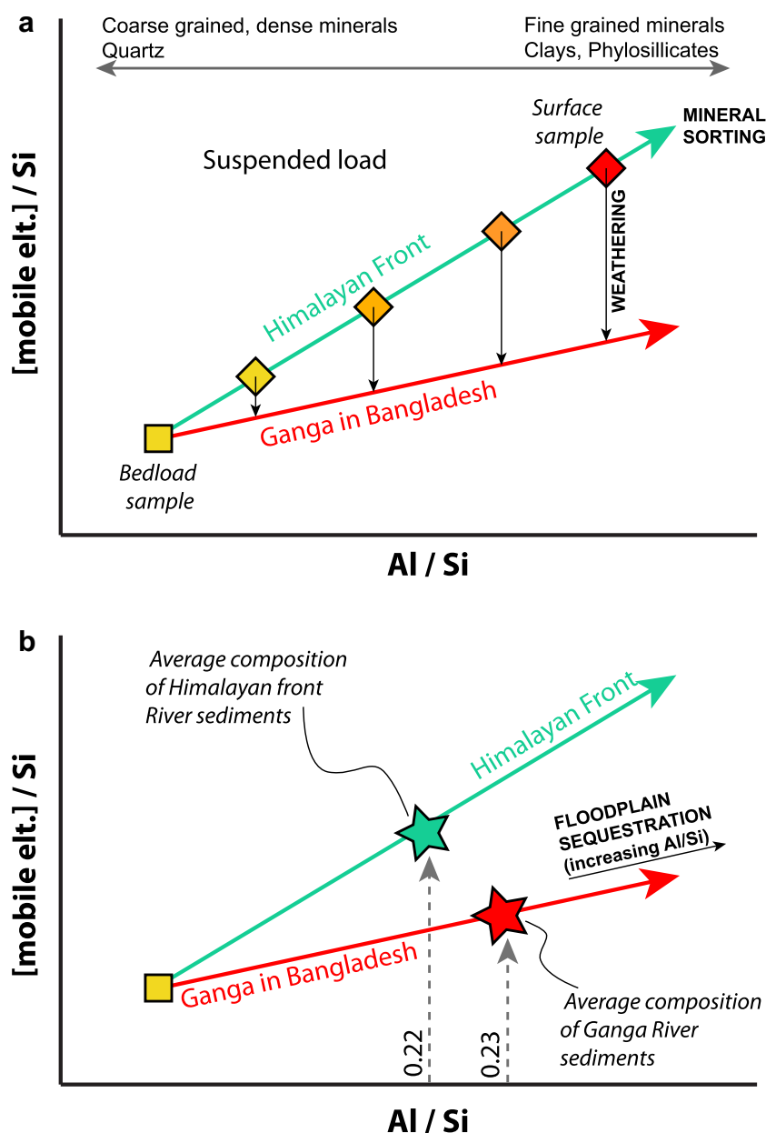
Fig. 3. Schematic evolution of the sedimentary load during transfer from the Himalayan front downstream to the Ganga in Bangladesh. (a) Sediment hydrodynamic sorting results in mixing trend between coarse grained, quartz rich, low Al/Si sediments and a clay and phyllosilicate rich end-member. Weathering is marked by a loss of mobile elements (e.g. K, Na,...) relative to Si at constant Al/Si. (b) Sediment sequestration in the floodplain results in a relative increase of the average Al/Si ratio of the total transported sediment load. This evolution is however limited for the Ganga as at the Himalayan front the average Al/Si is ca. 0.22 and in the Ganga in Bangladesh this ratio is estimated at ca. 0.23 (Lupker et al., 2011).
