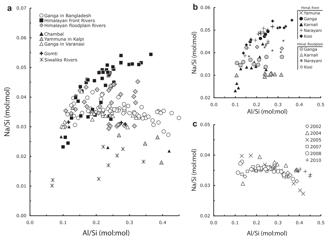
Fig. 5. (a) Evolution of the Na/Si ratio as a function of the Al/Si ratio, showing a depletion in Na relative to Si from the Himalayan front Rivers (black squares) downstream to the Himalayan floodplain Rivers (light gray diamonds) and the Ganga in Bangladesh (open circles). (b) Composition variability amongst Himalayan front Rivers showing a Na-depleted Karnali compared to other Himalayan Rivers. (c) Inter-annual variability of the Na/Si ratio in Ganga sediments sampled in Bangladesh.
