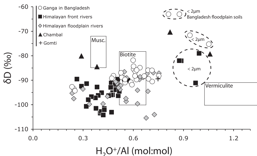
Fig. 8. D/H isotopic composition of bulk sediments from the Ganga basin as a function of hydration expressed as the \text{H}_2\text{O}^+/\text{Al} ratio. The hydration and isotopic composition of muscovite, biotite and vermiculite separated from Himalayan sediments (see Supplementary data file, Table S2 ) is also plotted for references.
