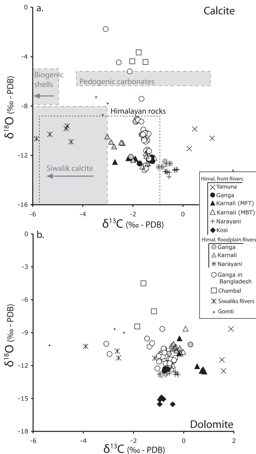
Fig. 10. Oxygen and carbon isotopic composition of calcite (a) and dolomite (b) of river sediments from the Ganga basin. The range of composition of pedogenic carbonates from the northeastern Ganga floodplain (Sinha et al., 2006), Siwaliks carbonates from the Surai Khola section in Nepal (Supplementary data file, Table S3; Sanyal et al., 2005), biogenic shells from the Gangetic plain (Gajurel et al., 2006) and Himalayan source rocks (Galy et al., 1999) is also shown.
