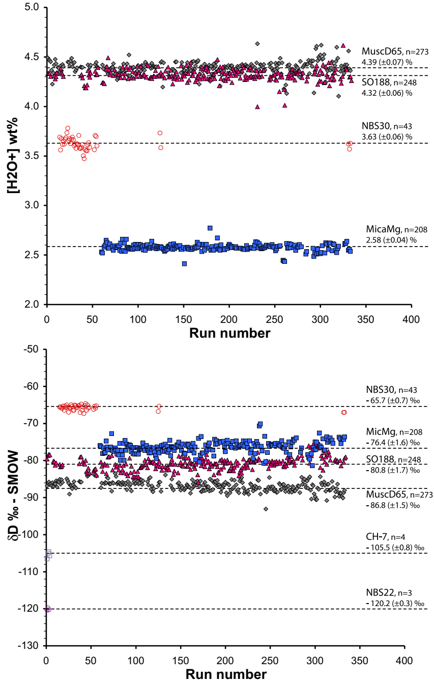
Fig. A1. Replicate analysis of internal standards MuscD65, Mica-Mg and SO188 for \text{H}_2\text{O}^+ concentration (top figure) and D/H isotopic composition (lower figure) routinely measured. Measurements of international reference (NBS 30, NBS 22 and CH-7) are also indicated.
