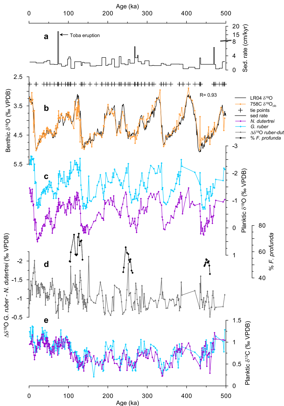
Fig. 2. ODP Hole 758C age model and palaeoclimate records. (a) Sedimentation rates and age tie points (crosses), (b) Site 758 C. wuellerstorfi \delta^{18}\text{O} record (orange) and the LR04 benthic foraminiferal \delta^{18}\text{O} stack (black, Lisiecki and Raymo, 2005), (c) Site 758 planktic \delta^{18}\text{O} records: G. ruber (blue) and N. dutertrei (purple), (d) Site 758 \Delta\delta^{18}\text{O}_{\text{r-d}} record (grey, maximum stratification plotted up) and percent F. profunda coccoliths (black, minimum productivity plotted up) and (e) Site 758 planktic \delta^{13}\text{C} records: G. ruber (blue) and N. dutertrei (purple). (For interpretation of the references to colour in this figure legend, the reader is referred to the web version of this article.)
