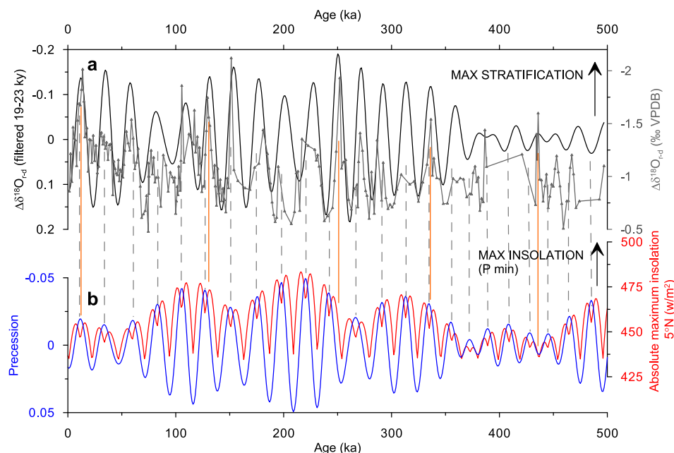
Fig. 5. Site 758 stratification compared to insolation forcing. (a) Site 758 \Delta\delta^{18}O_{r-d} record (maximum stratification plotted up), raw (grey) and filtered to illustrate only variance at the 19 and 23 ka precession periods (black; filter: frequency 0.045, bandwidth 0.008). (b) Precession (blue) and absolute maximum insolation at 5°N (red) (Huybers, 2006). Grey dotted lines illustrate P minima, solid orange lines indicate the five stratification peaks that occur at the onset of glacial terminations. (For interpretation of the references to colour in this figure legend, the reader is referred to the web version of this article.)
