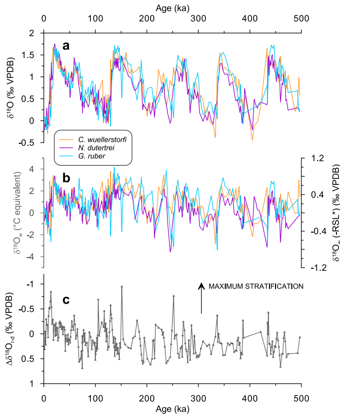
Fig. 6. \delta^{18}\text{O} records for Site 758. (a) Site 758 \delta^{18}\text{O} records for the three foraminiferal species (colours as in Fig. 2). (b) Site 758 \delta^{18}\text{O} records for the three foraminiferal species minus variance attributed to global sea level change. The sea level component was removed by subtracting the Red Sea relative sea level curve of Rohling et al. (2009a, 2010) rescaled to the age scales of the Site 758 records, from foraminiferal \delta^{18}\text{O} assuming a 0.01\text{‰} change in \delta^{18}\text{O} per metre of sea level change (Adkins and Schrag, 2001). The local temperature component was not subtracted because no sea surface temperature (SST) record exists for our site; therefore, the resultant \delta^{18}\text{O}_w records include local SST and salinity components. (c) Site 758 \Delta\delta^{18}\text{O}_{R-d} record (maximum stratification plotted up). All data are normalised to mean values for 0–6 ka and plotted with positive values up except \Delta\delta^{18}\text{O}_{R-d} , which has an inverted axis so that maximum stratification points up.
