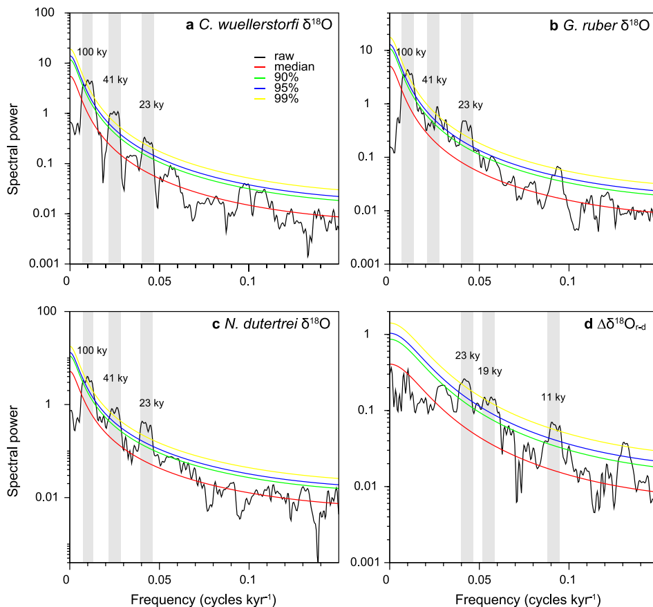
Fig. 3. Spectral power versus frequency plots for Site 758 \delta^{18}\text{O} records. (a) C. wuellerstorfi , (b) G. ruber , (c) N. dutertrei and (d) \Delta\delta^{18}\text{O}_{\text{r-d}} . Significant orbital frequencies are highlighted.
