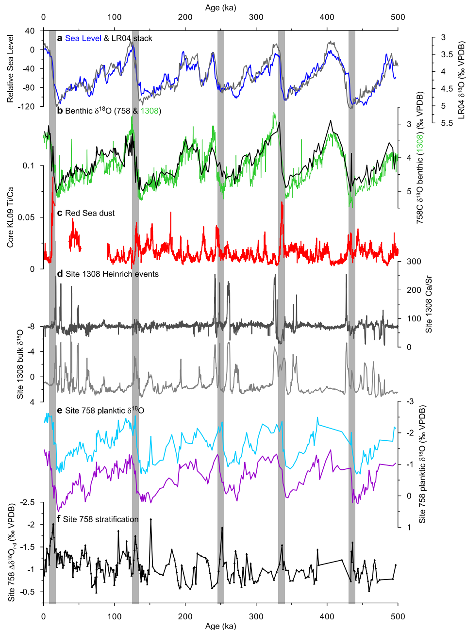
Fig. 8. Correlation of terminal stratification peaks at Site 758 with remote millennial-scale climate events. (a) Red Sea relative sea level record, 1 ka Gaussian smoothing applied (blue; Rohling et al., 2009a,b, 2010) and the LR04 benthic foraminiferal \delta^{18}\text{O} stack (black; Lisiecki and Raymo, 2005), (b) benthic foraminiferal \delta^{18}\text{O} records for Site 758 (black; this study) and Site 1308 (green; Hodell et al., 2008), (c) Red Sea dust proxy record (Ti/Ca), 1 ka Gaussian smoothing applied (Roberts et al., 2011), (d) IODP Site 1308 North Atlantic ice-rafted debris proxy records, Ca/Sr ratios and bulk sediment \delta^{18}\text{O} (Hodell et al., 2008), (e) Site 758 planktic foraminiferal \delta^{18}\text{O} records and (f) Site 758 \Delta\delta^{18}\text{O}_{\text{e-o}} record (maximum stratification plotted up). Grey bands highlight stratification peaks at glacial terminations. (For interpretation of the references to colour in this figure legend, the reader is referred to the web version of this article.)
