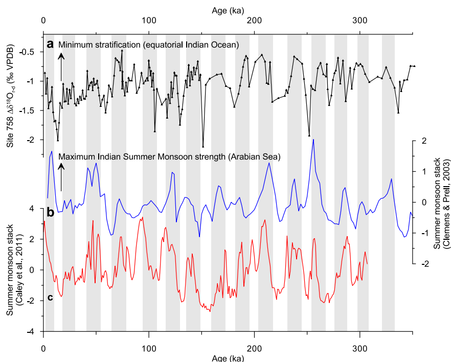
Fig. 7. Comparison of the Site 758 stratification record with two Arabian Sea summer monsoon stacks. (a) Site 758 \Delta\delta^{18}\text{O}_{\text{e-o}} record (minimum stratification plotted up), (b) Arabian Sea summer monsoon stack (Clemens and Prell, 2003), and (c) Arabian Sea summer monsoon stack (Caley et al., 2011b).
