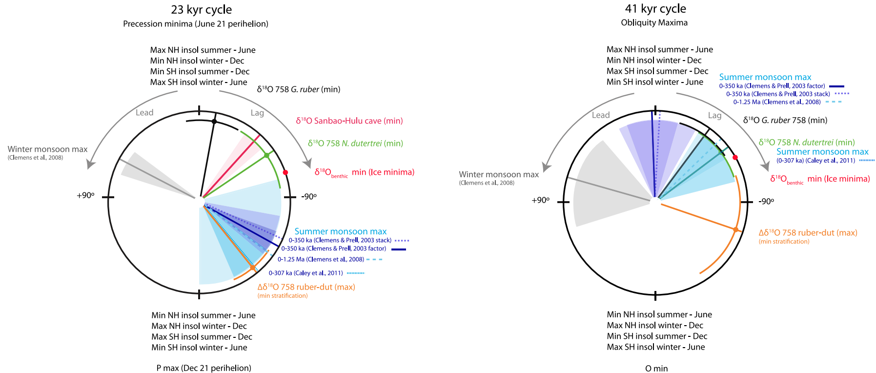
Fig. 4. Phase wheels summarizing the late Pleistocene monsoon response to insolation forcing at the orbital precession (23 ka) and obliquity (41 ka) periods. The precession index is defined as \Delta \sin \omega where \omega is the longitude of the perihelion measured from the moving vernal point and e is the eccentricity of Earth's orbit about the Sun (Berger and Loutre, 1977; Laskar et al., 1993). Obliquity is the tilt of Earth's axis with respect to the ecliptic plane. Zero phase is set to precession minima (P min; \omega = 90^\circ , 21st June perihelion) and obliquity maxima (O max), respectively. Negative phases are measured in the clockwise direction and represent phase lags relative to P min or O max. Positive phases are measured in the anticlockwise direction and represent phase leads relative to P min or O max. Phase relationships of ice volume are also shown (red dots, Lisiecki and Raymo, 2005). All Site 758 isotope records are coherent with Site 758 \delta^{18}\text{O}_{\text{benthic}} at the 95% confidence level except \Delta \delta^{18}\text{O}_{\text{r-d}} at the obliquity period (80% confidence level) (Table 1). Published records plotted (with shaded phase estimate errors) are the Arabian Sea summer monsoon stack (Caley et al., 2011b), the Arabian Sea summer monsoon stack and summer monsoon factor (Clemens and Prell, 2003), the Chinese Sanbao-Hulu composite cave \delta^{18}\text{O} (Cheng et al., 2009), and winter and summer monsoon maxima (Clemens et al., 2008). NH = northern hemisphere, SH = southern hemisphere. (For interpretation of the references to colour in this figure legend, the reader is referred to the web version of this article.)
