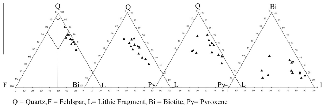
Fig. 7. On a Q (quartz)–F (feldspar)–L (lithic fragment) diagram, the Mujpur samples plot as sublitharenite. Basalt fragments mostly represent lithics in the samples; pyroxene and biotite representing other mafic phases.
