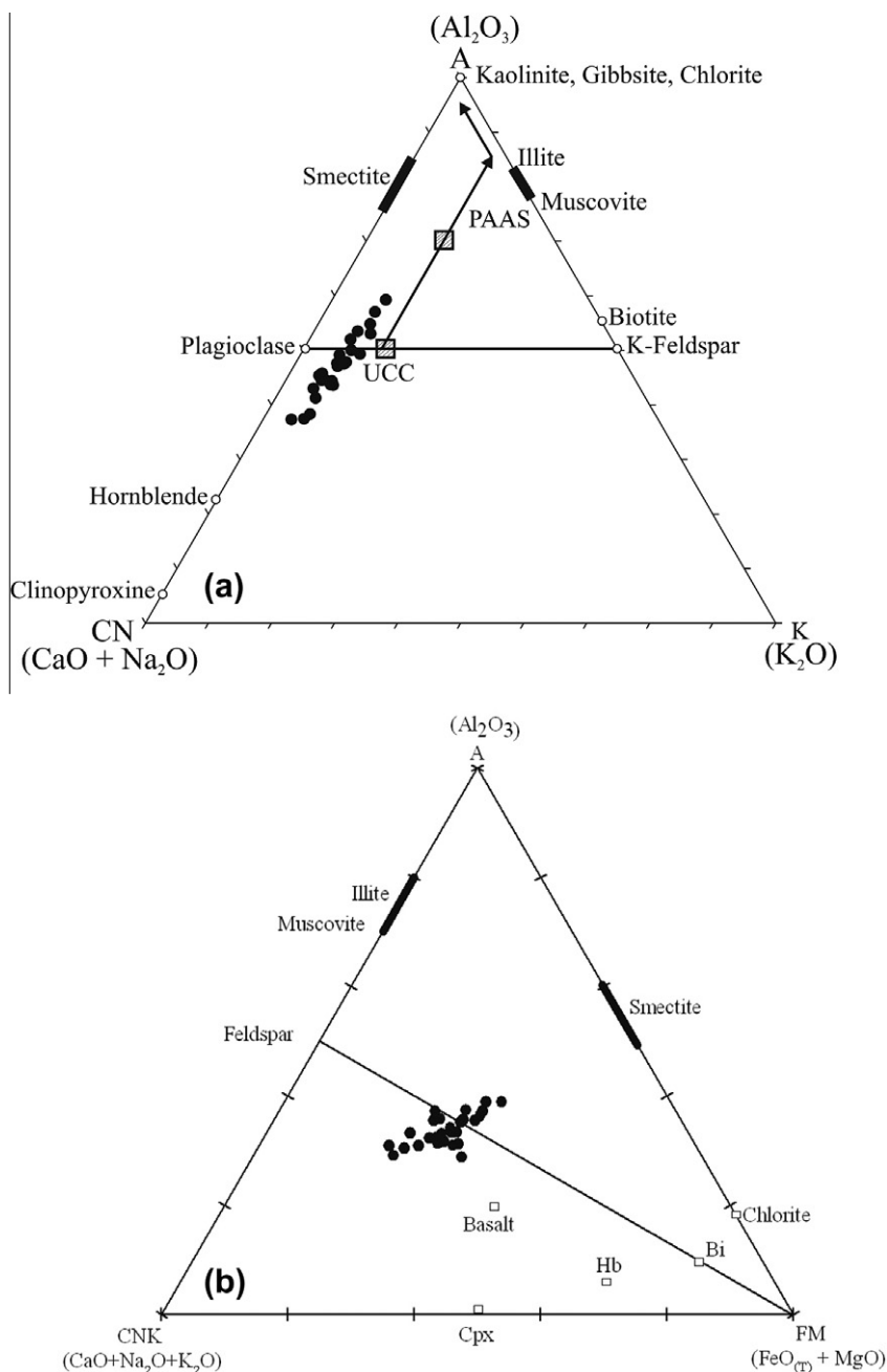
Fig. 12. Triangular (a) A–CN–K (b) A–CNK–FM plots of the Muppur samples (for calculations of A, C, N, K, F and M components, see in text). (a) Samples plot at or about UCC; few samples plot even below upper continental crust (UCC: CIA = ~50) indicating presence of mafic components. (b) In A–CNK–FM plot, samples cluster halfway of feldspar–biotite join closer to field of basalt, consistent with presence of basalt fragments in the samples.
