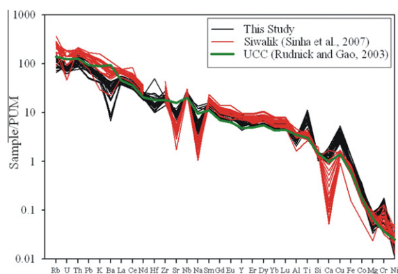
Fig. 14. Multi-element primitive upper mantle (PUM)-normalized pattern for the Mujpur and Siwalik samples. Note that the Siwalik siltstone are enriched in LIL and rare earth elements, but depleted in more compatible elements (Cr, Co, Cu) in comparison to the Mujpur alluvial samples. The negative anomalies of Ba, Sr, Na and Ca are characteristics of both plots (see text for details). Upper continental crust (UCC: Rudnick and Gao, 2003) is plotted for comparison. Composition of the Siwalik rocks from Sinha et al. (2007). PUM (primitive upper mantle) taken from Palme and O'Neill (2003).
