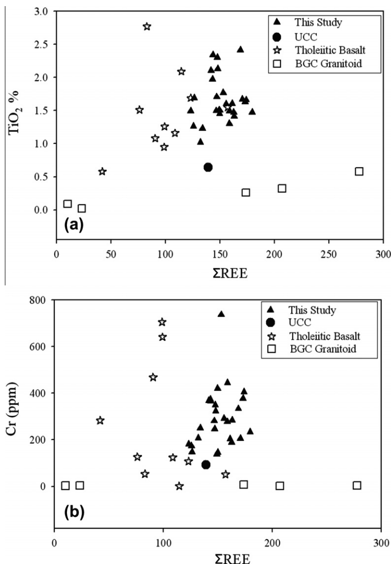
Fig. 10. (a) Total REE ( \Sigma\text{REE} ) vs. \text{TiO}_2 (wt.%) plot showing comparable or slightly lesser total REE concentrations in samples and Tholeiitic basalt (Ahmad and Tarney, 1994) at given \text{TiO}_2 (1–2.4 wt.%). Note granitoid (Ahmad and Tarney, 1994) have larger spread in REE concentrations at a given \text{TiO}_2 (0.05 wt.%). (b) Total REE ( \Sigma\text{REE} ) vs. Cr (ppm) plot showing similar Cr (200–400 ppm) samples and Tholeiitic basalt. Granitoid have large spread in total REE values at a much lesser Cr concentration ( \sim <10 ppm).
