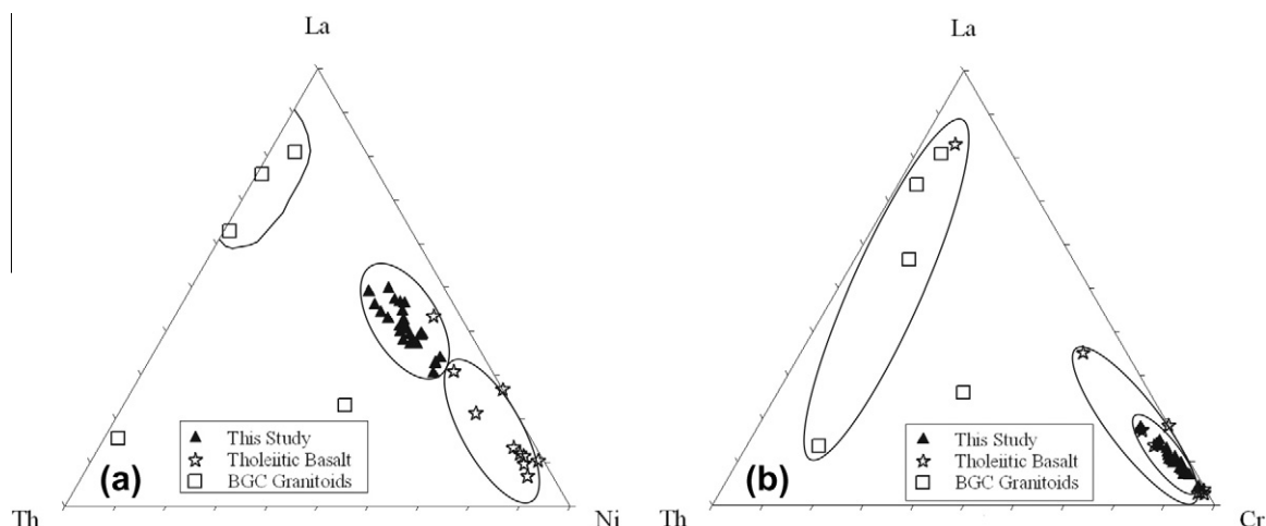
Fig. 13. (a) Th–La–Ni diagram showing samples plot towards La–Ni side, but clearly away from Th (felsic source), (b) Mujpur samples plot within the field of tholeiite basalt. Sources: Tholeiitic basalt and granitoid (Ahmad and Tarney, 1994).
