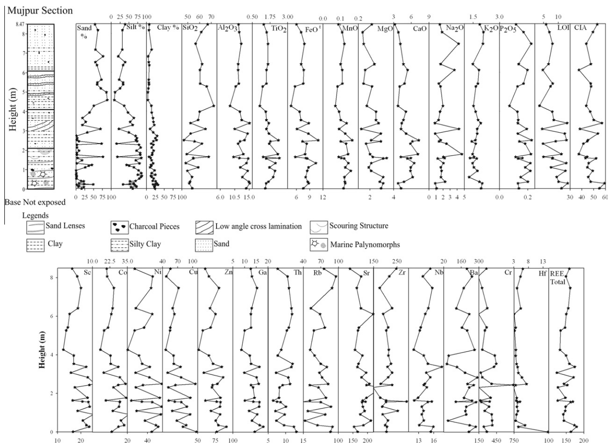
Fig. 4. Grain size (sand, silt \pm clay) distributions in the Mujpur profile along with the litholog. Note that \text{SiO}_2 and felsic components are more in the coarser mode (coarse sand) whereas mafic components are enriched in the finer sediments.
